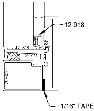
1" GLAZING
