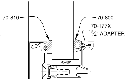
7/8" GLAZING
