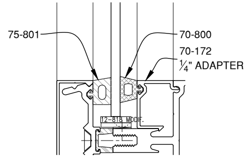
3/16" GLAZING
