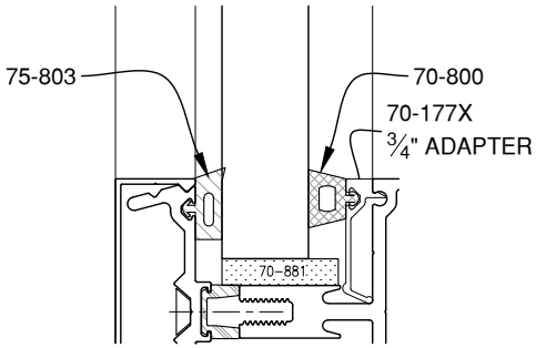
13/16" GLAZING
