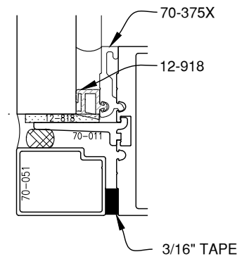
7/8" GLAZING
