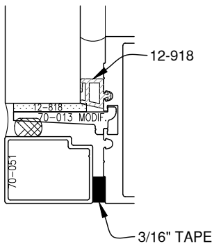
1 1/8" GLAZING
