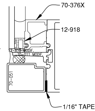
3/16" GLAZING
