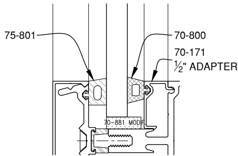
7/16" GLAZING
