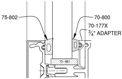
13/16" GLAZING
