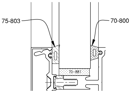
1 1/8" GLAZING
