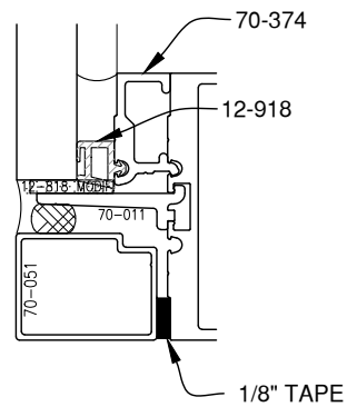
9/16" GLAZING
