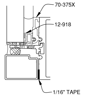
11/16" GLAZING
