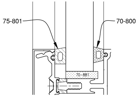
15/16" GLAZING
