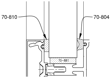
1 3/16" GLAZING
