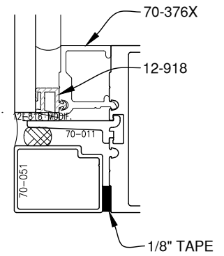
5/16" GLAZING
