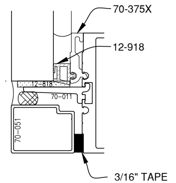
7/8" GLAZING
