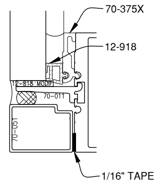
3/4" GLAZING
