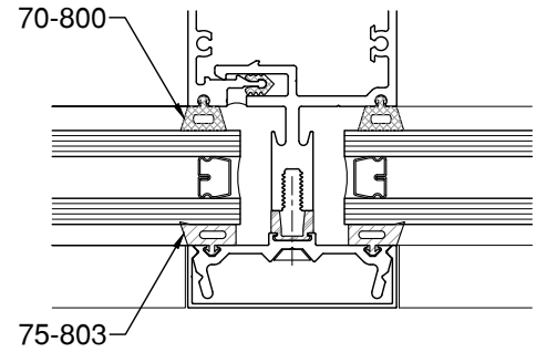
1 1/8" GLAZING
