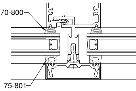
1" GLAZING
