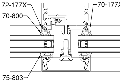
7/8" GLAZING
