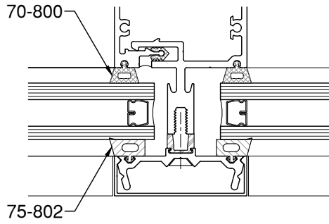
1 1/16" GLAZING
