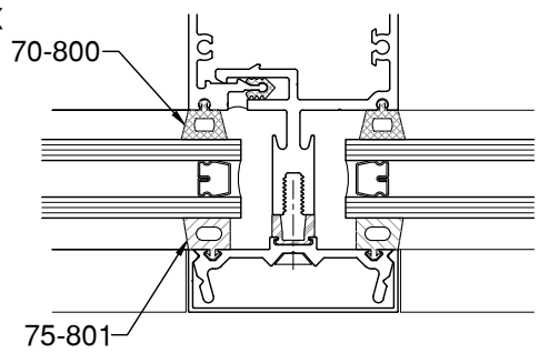
15/16" GLAZING
