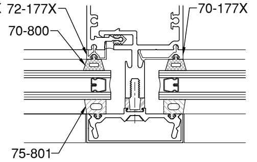
3/4" GLAZING
