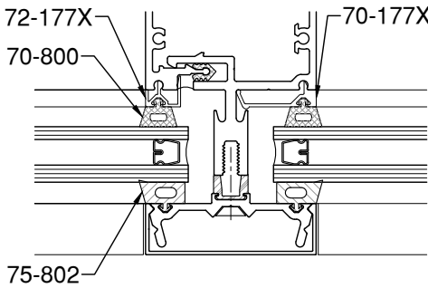
13/16" GLAZING
