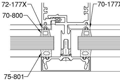
11/16" GLAZING
