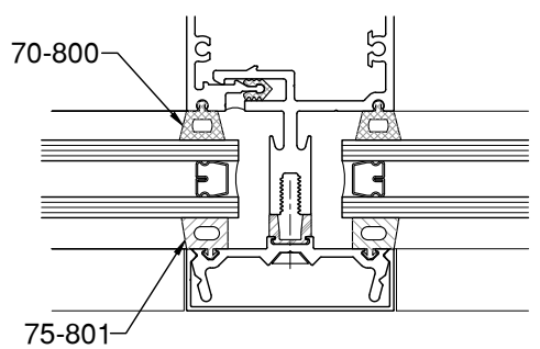
15/16" GLAZING
