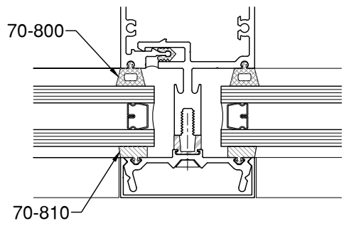
1 1/8" GLAZING
