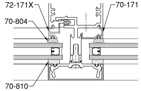
3/4" GLAZING
