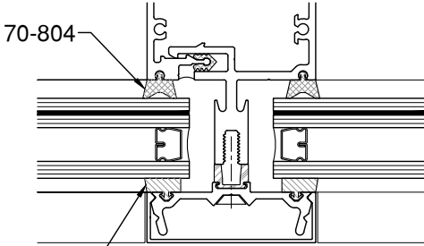
1 3/16" GLAZING
