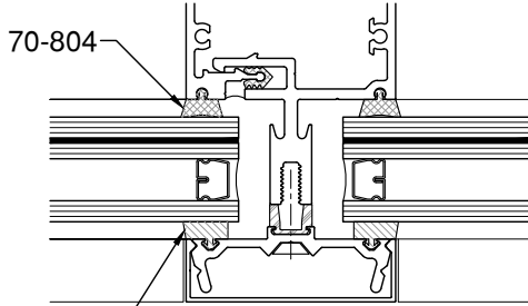
1 1/4" GLAZING
