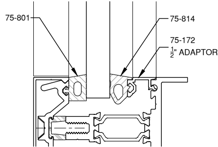
1/2" GLAZING
