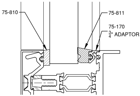
15/16" GLAZING
