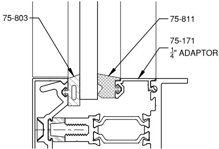
3/8" GLAZING
