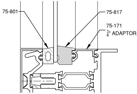
1/8" GLAZING
