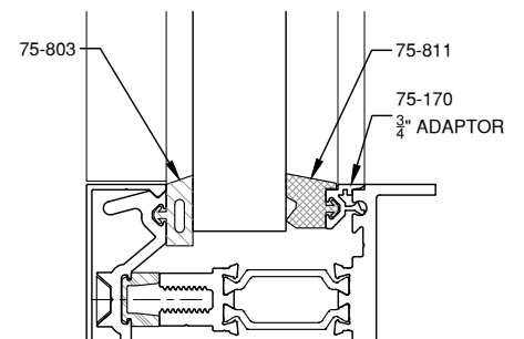
7/8" GLAZING
