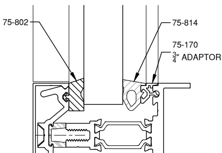
13/16" GLAZING
