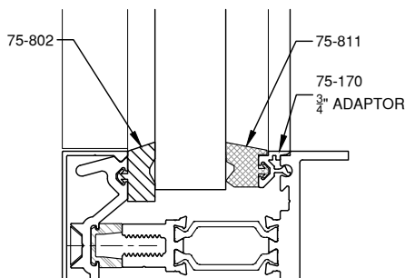
13/16" GLAZING
