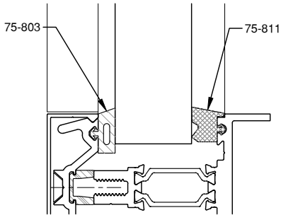
1 1/8" GLAZING
