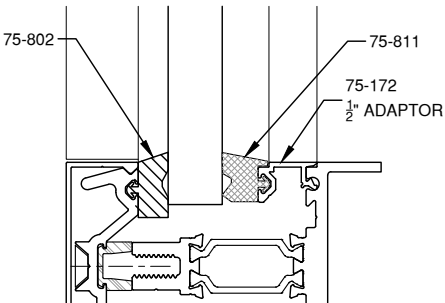
9/16" GLAZING
