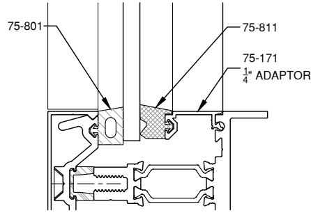
1/4" GLAZING
