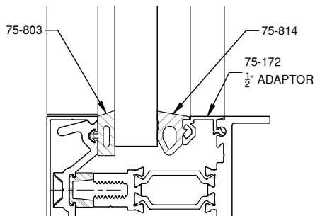
5/8" GLAZING
