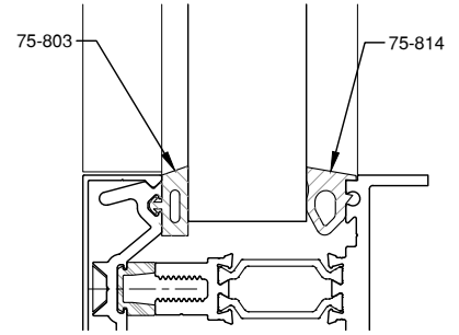
1 1/8" GLAZING
