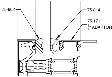
5/16" GLAZING
