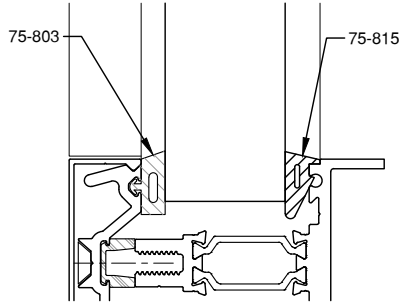
1 1/4" GLAZING
