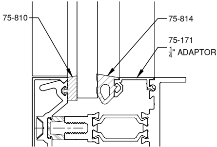
7/16" GLAZING
