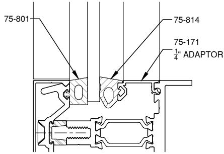
1/4" GLAZING
