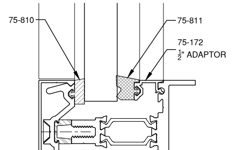
11/16" GLAZING
