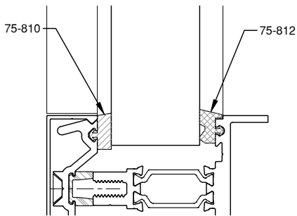
1 5/16" GLAZING
