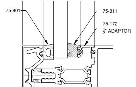
1/2" GLAZING
