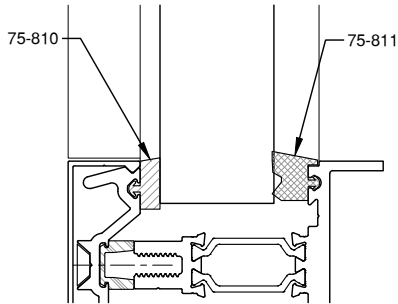
1 3/16" GLAZING
