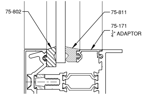
5/16" GLAZING
