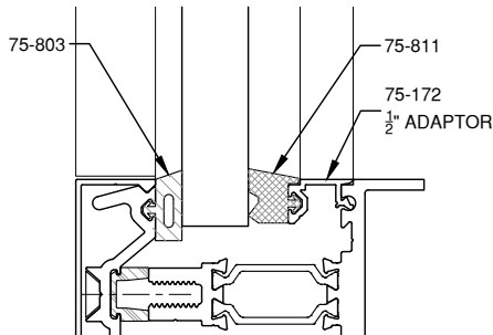
5/8" GLAZING
