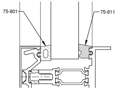
1" GLAZING
