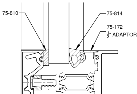
11/16" GLAZING
