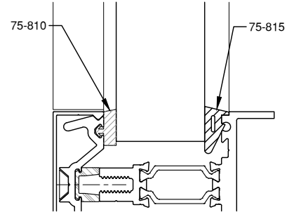
1 5/16" GLAZING
