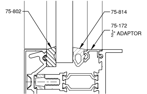
9/16" GLAZING
