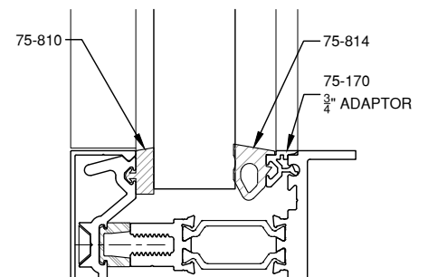
15/16" GLAZING
