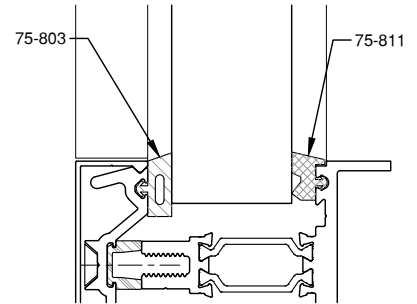
1 1/4" GLAZING
