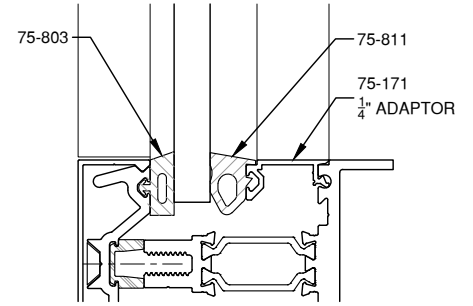
3/8" GLAZING
