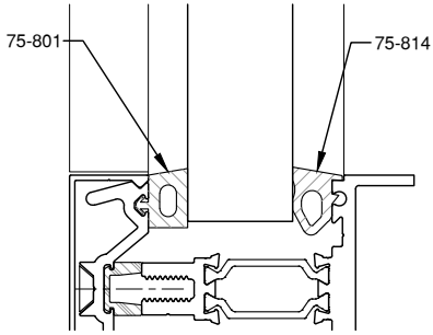
1" GLAZING
