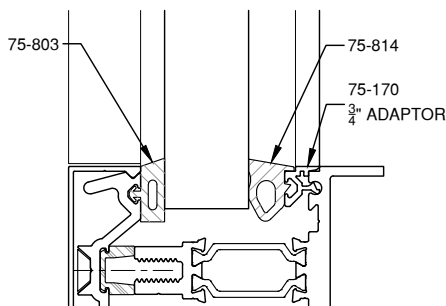
7/8" GLAZING
