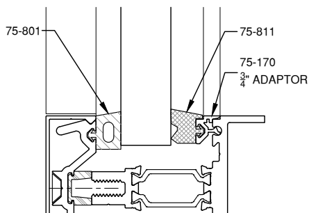
3/4" GLAZING
