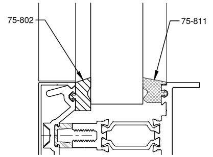
1 1/16" GLAZING
