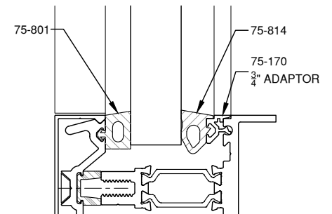
3/4" GLAZING
