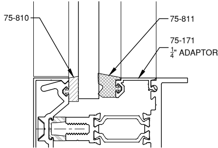
7/16" GLAZING
