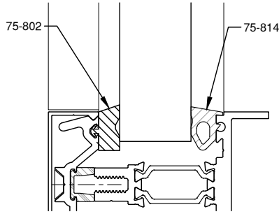
1 1/16" GLAZING
