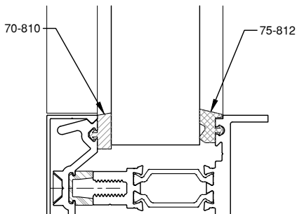
1 5/16" GLAZING
