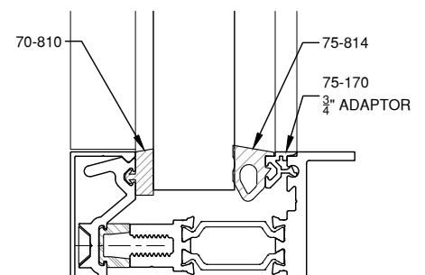
15/16" GLAZING
