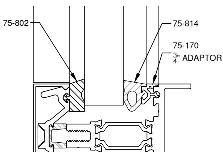
13/16" GLAZING
