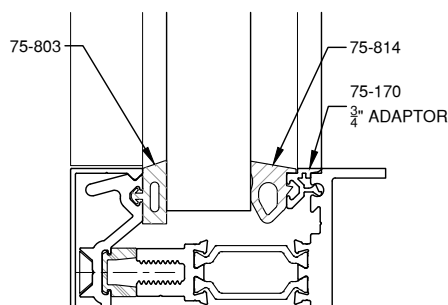
7/8" GLAZING
