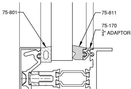
3/4" GLAZING
