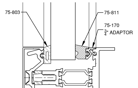
7/8" GLAZING
