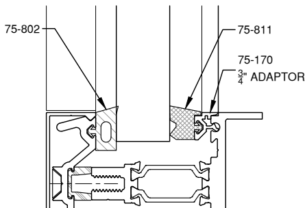
13/16" GLAZING
