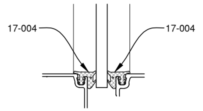
1/4" GLAZING
