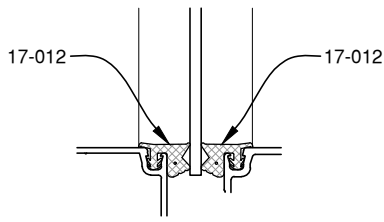
1/8" GLAZING
