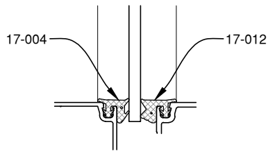
3/16" GLAZING
