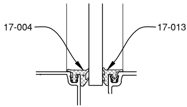
5/16" GLAZING
