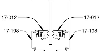
1/8" GLAZING
