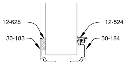
1 1/8" GLAZING
