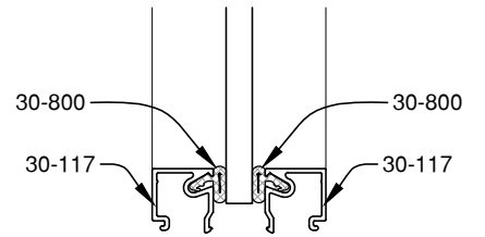
1/4" GLAZING
