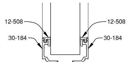
1 1/16" GLAZING
