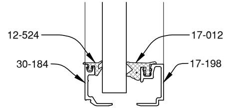
1/2" GLAZING
