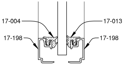
5/16" GLAZING
