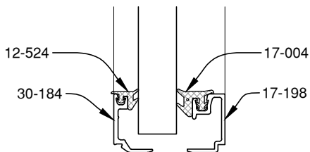
5/8" GLAZING
