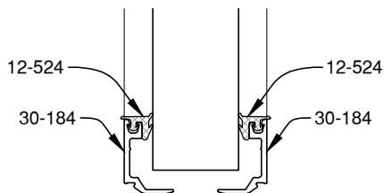
1" GLAZING
