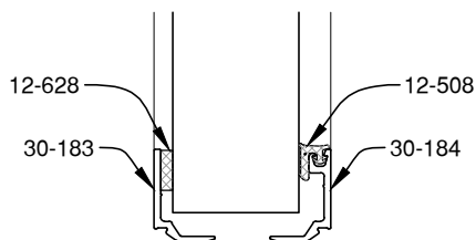
1 3/16" GLAZING
