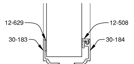
1 1/4" GLAZING
