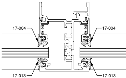
7/16" GLAZING 19-045 1/4" GLAZING ADAPTOR 17-004 INTERIOR GASKET 17-013 EXTERIOR GASKET
