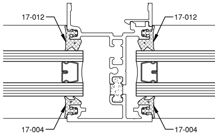
1 1/16" GLAZING 17-012 INTERIOR GASKET 17-004 EXTERIOR GASKET
