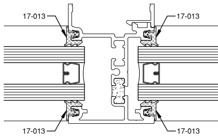
1 1/4" GLAZING 17-013 INTERIOR GASKET 17-013 EXTERIOR GASKET
