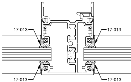
1/2" GLAZING 19-045 1/4" GLAZING ADAPTOR 17-013 INTERIOR GASKET 17-013 EXTERIOR GASKET
