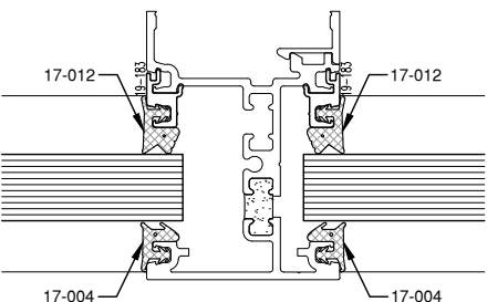
11/16" GLAZING 19-183 5/8" GLAZING ADAPTOR 17-012 INTERIOR GASKET 17-004 EXTERIOR GASKET
