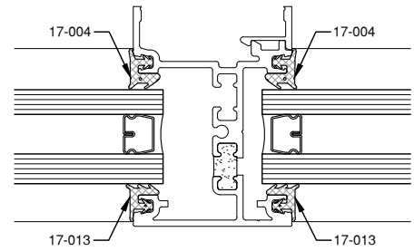
1 3/16" GLAZING 17-004 INTERIOR GASKET 17-013 EXTERIOR GASKET
