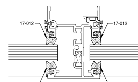
5/8" GLAZING 19-183 5/8" GLAZING ADAPTOR 17-012 INTERIOR GASKET 17-012 EXTERIOR GASKET
