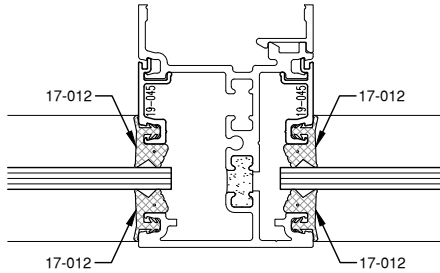
1/4" GLAZING 19-045 1/4" GLAZING ADAPTOR 17-012 INTERIOR GASKET 17-012 EXTERIOR GASKET
