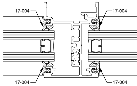
1 1/8" GLAZING 17-004 INTERIOR GASKET 17-004 EXTERIOR GASKET
