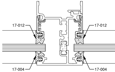
5/16" GLAZING 19-045 1/4" GLAZING ADAPTOR 17-012 INTERIOR GASKET 17-004 EXTERIOR GASKET
