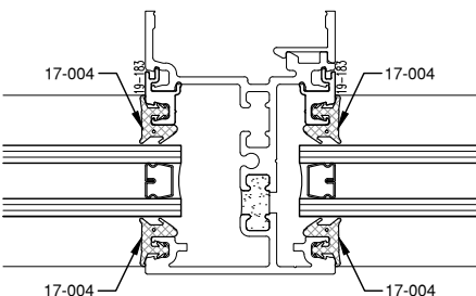
3/4" GLAZING 19-183 5/8" GLAZING ADAPTOR 17-004 INTERIOR GASKET 17-004 EXTERIOR GASKET
