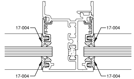
3/8" GLAZING 19-045 1/4" GLAZING ADAPTOR 17-004 INTERIOR GASKET 17-004 EXTERIOR GASKET
