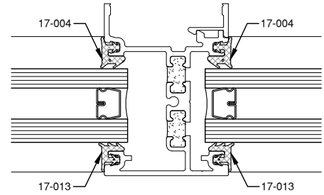
1 3/16" GLAZING 17-004 INTERIOR GASKET 17-013 EXTERIOR GASKET
