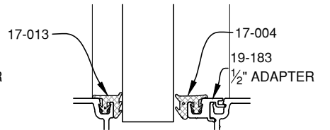
13/16" GLAZING
