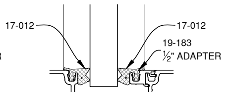
5/8" GLAZING
