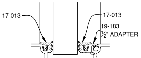
7/8" GLAZING
