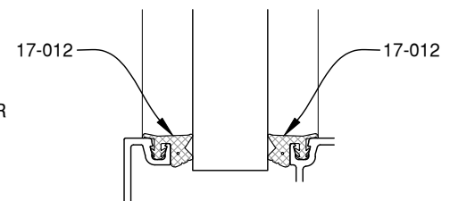
7/8" GLAZING
