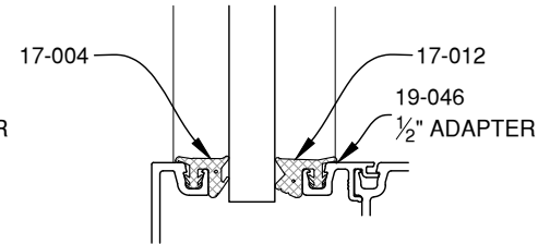
7/16" GLAZING
