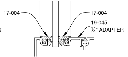
1/4" GLAZING
