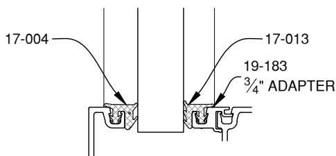
11/16" GLAZING
