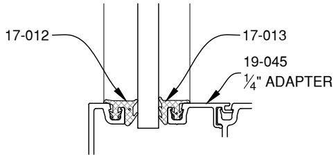
5/16" GLAZING
