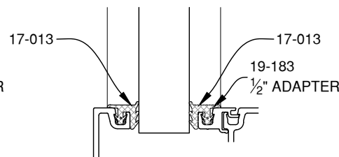
3/4" GLAZING
