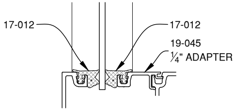
1/8" GLAZING
