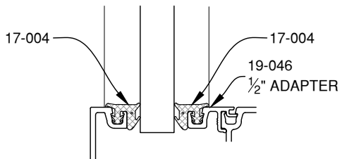
1/2" GLAZING
