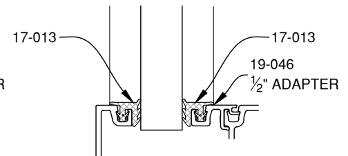
5/8" GLAZING
