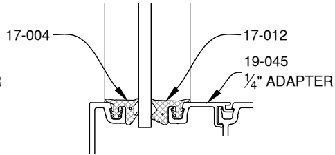
3/16" GLAZING
